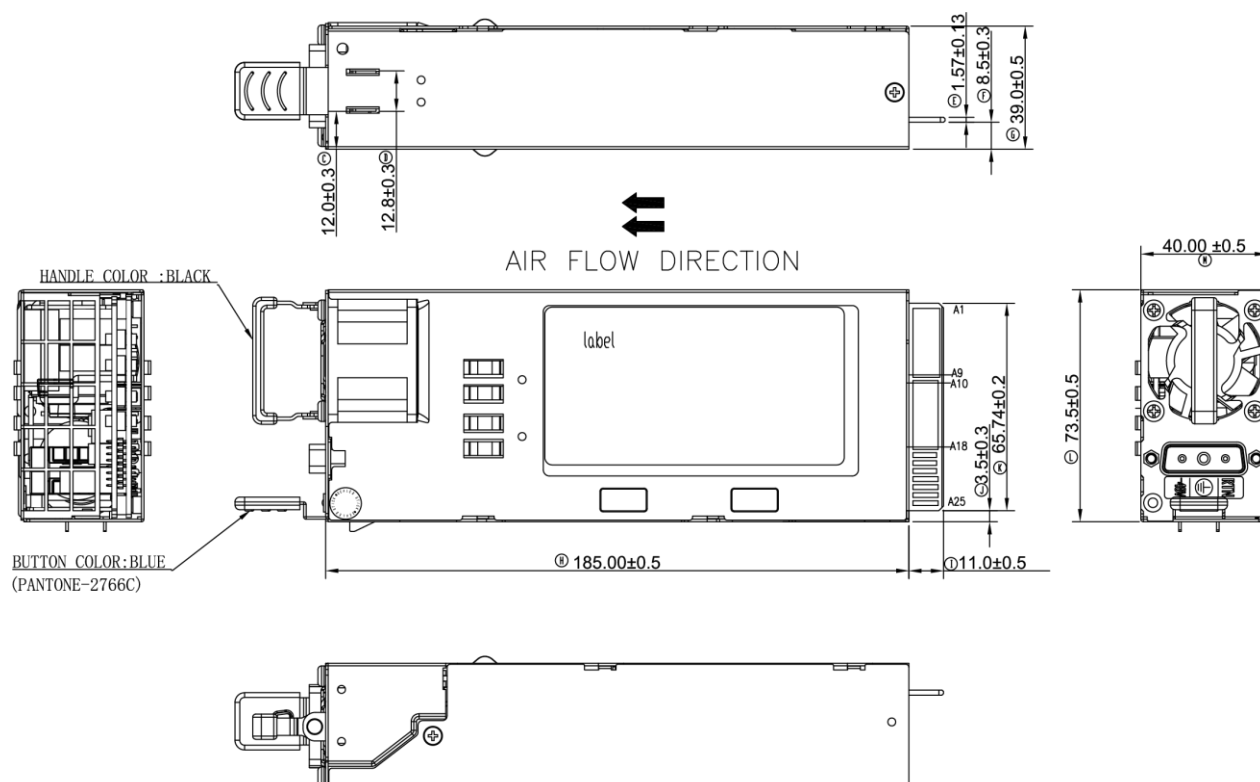
Figure 5. Mechanical Drawing
