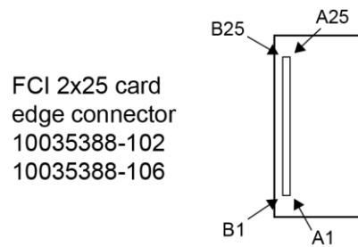
Figure 8. Back DC output golden finger port
